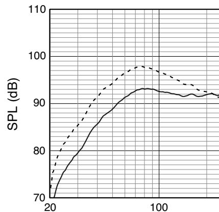
Frequency Response:
