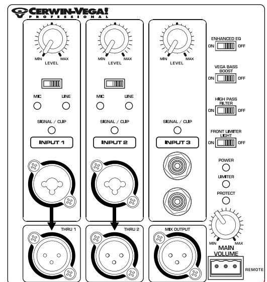
Rear Panel - P1000X and P1500X
