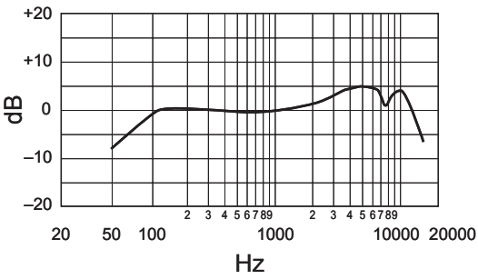
Frequency Response
