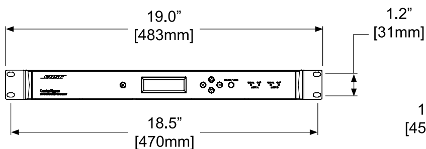
Front View
