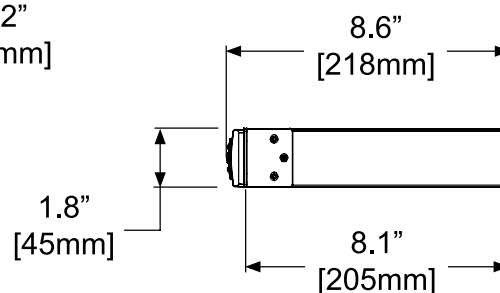
Right View
