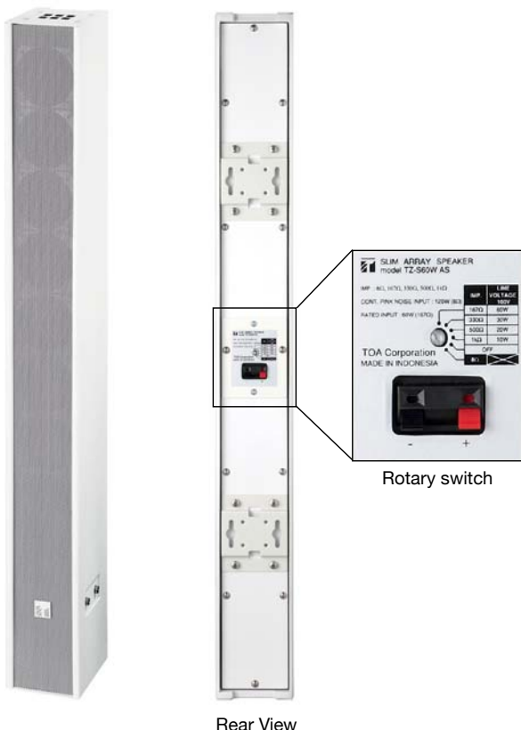
Rear View
